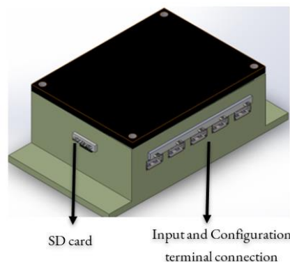
Figure 3. Design layout on the data logger module.
