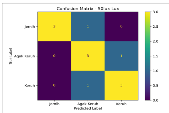
Gambar 7. Confusion Matrix 50 Lux
