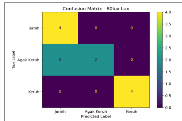
Gambar 6. Confusion Matrix 80 Lux
